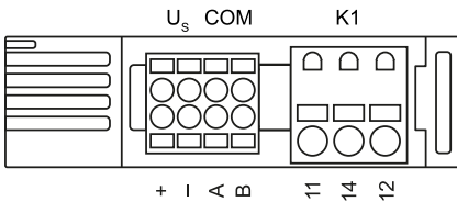
Figure 4-2: isoGEN413R-1 bottom
