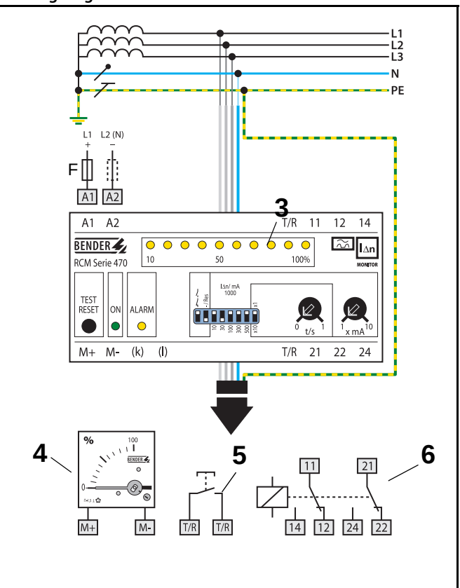
Wiring diagram
