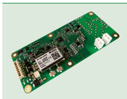
ISOMETER® IR155-4204
