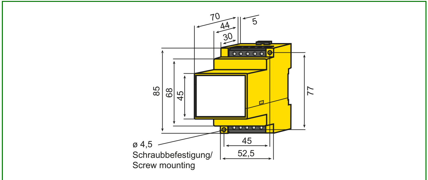
Fig. 1: Dimension diagram; all dimensions in mm
